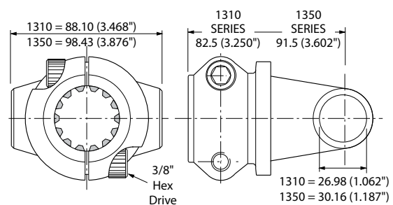
INTEGRAL CLAMPLOCK YOKES
