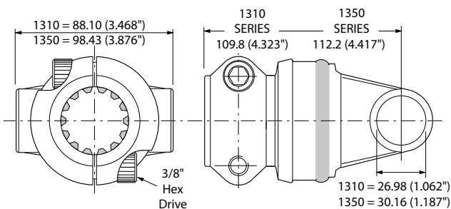
CLAMPLOCK YOKES
