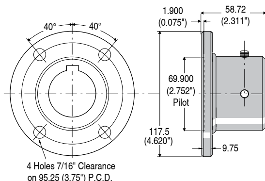
ROUND BORE SERIES - 1350 & 1410 Spicer
